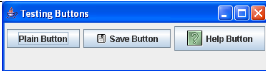
Initial GUI
